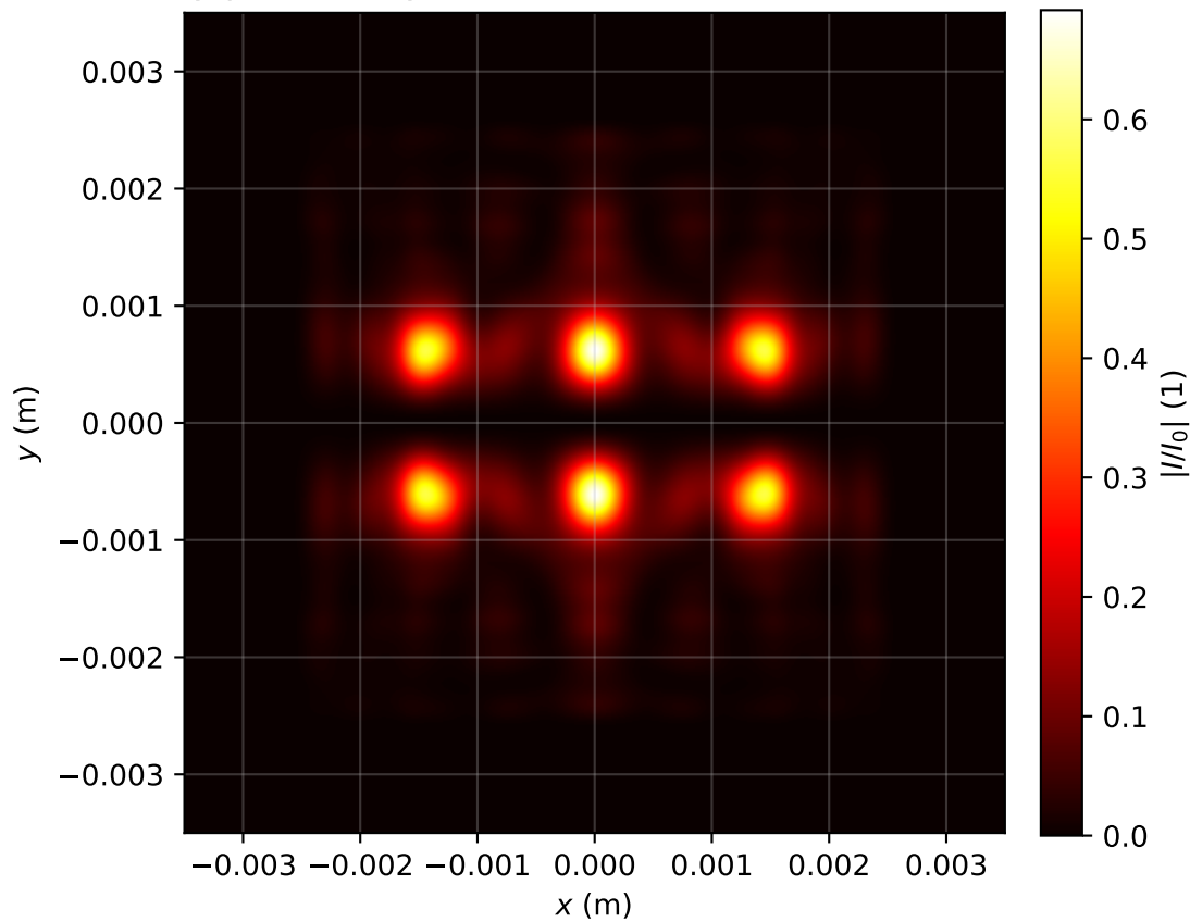
Intensity profile I(x, y, z = 3.025)/I_0 , P_{in}=5.0P_{cr} , artificial time
